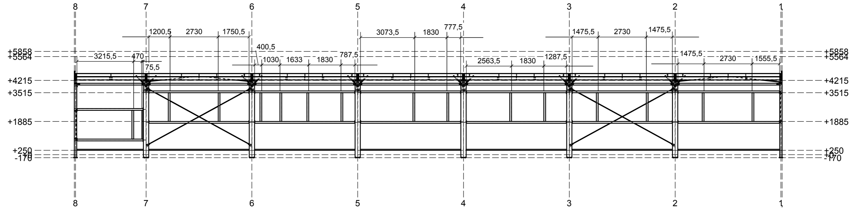
View 07 (+0) 1:125
