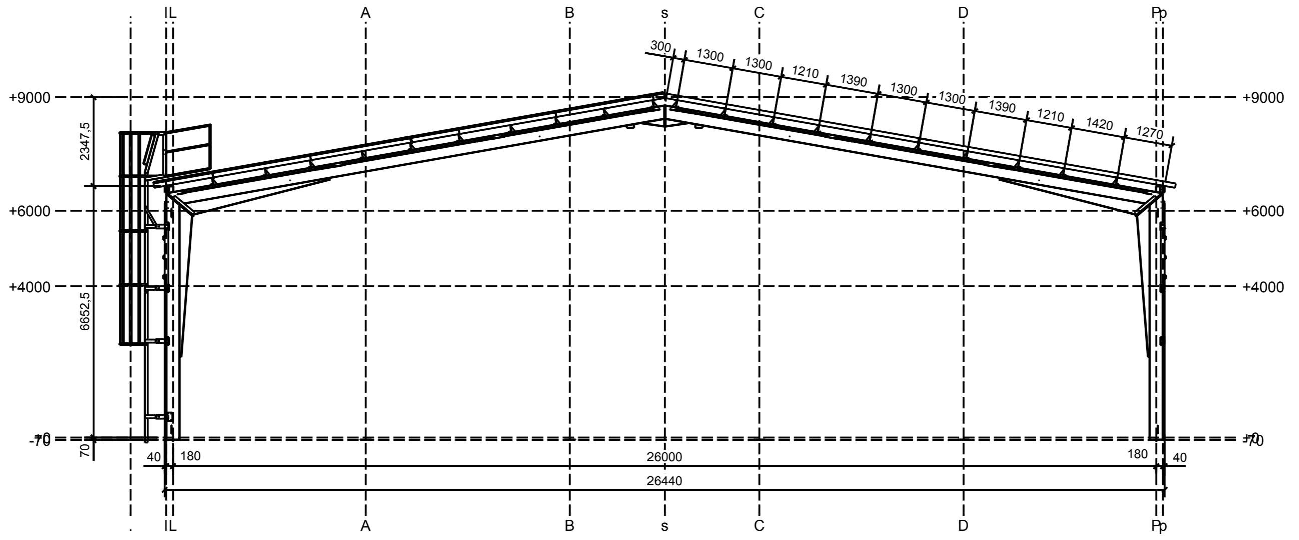
AXIS 2 1:100
